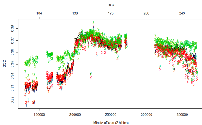
Fig. 1. Webcam results from Tammela year 2014, showing a distinct springtime increase in the greenness index (gcc).
