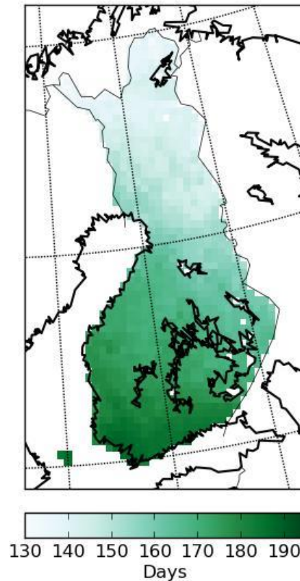
Fig. 2. Vegetation active period according to JSBACH model results.
